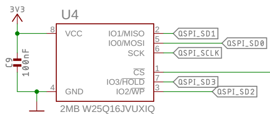
Flash memory
