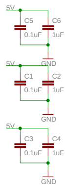
Matrix Driver Decoupling
