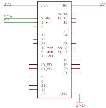
Raspberry Pi GPIO
