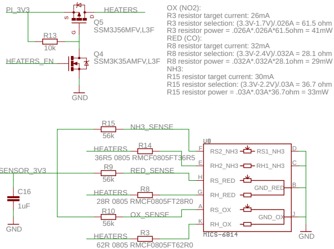
MICS-6814 Analog NO2 & CO & NH3 Sensor
