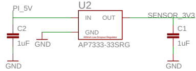
5V -> 3V3 LDO Regulator for sensors
