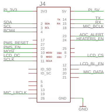
Pi GPIO connector
