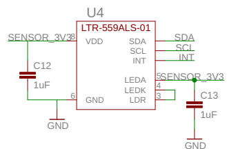
LTR-559 digital light sensor
