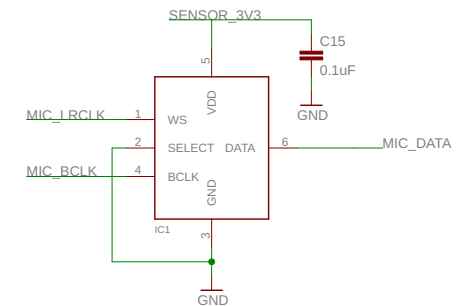
Digital I2S microphone
