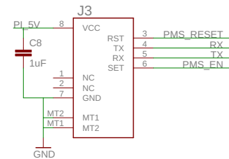
Connection for PMS5003 / 7003 PM Sensor
