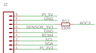
I2C & ADC extension header, unpopulated Breakout Garden Pinout
