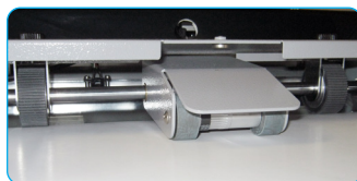
High-capacity feeder with three feed rollers plus two auxiliary feed wheels for consistent feeding
