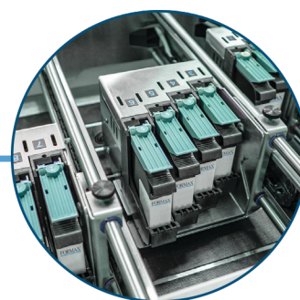
2 + 4 + 2 Stitched Print Heads Three independent print heads for 8 high-capacity inkjet cartridges
