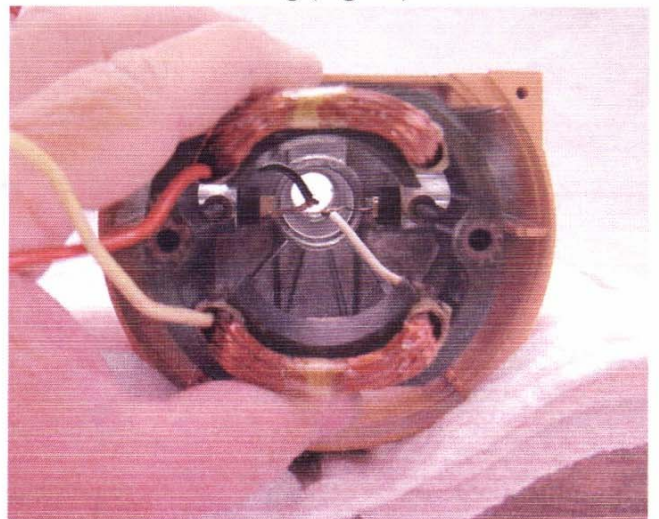
Fig. 36 Positioning the stator on the two stator studs and into the ribs of the motor housing.
