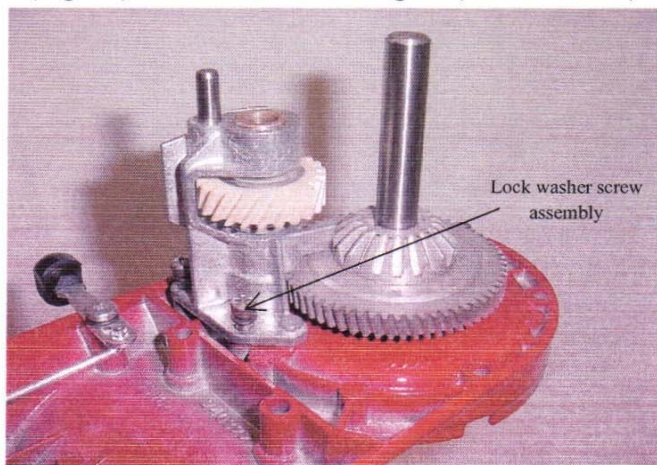
Fig. 59 Secure the three lock washer screw assemblies into the bottom cover.
