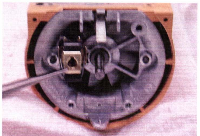
Fig. 22 Governor shown removed from the shaft of the motor.
