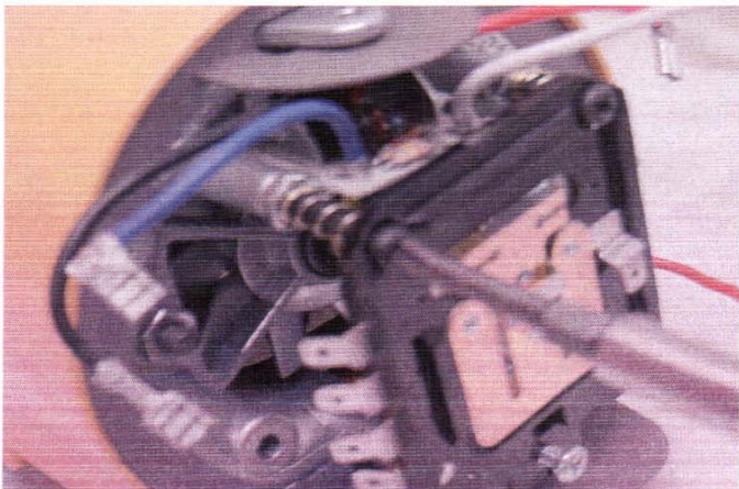
Fig. 49 Placing the control board on the bearing bracket.
