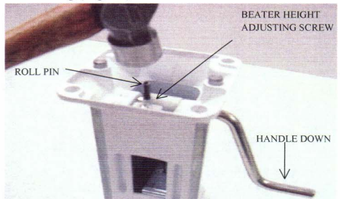
Fig. 91 The roll pin is driven in until it is almost flush with the arm. While the adjusting screw is replaced from this side, it is adjusted from the other.
