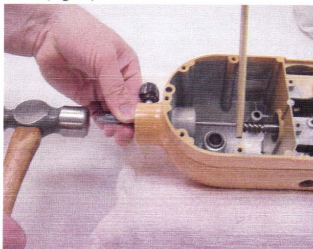
Fig. 30 A block of wood is used to protect the motor shaft when removing the armature.
