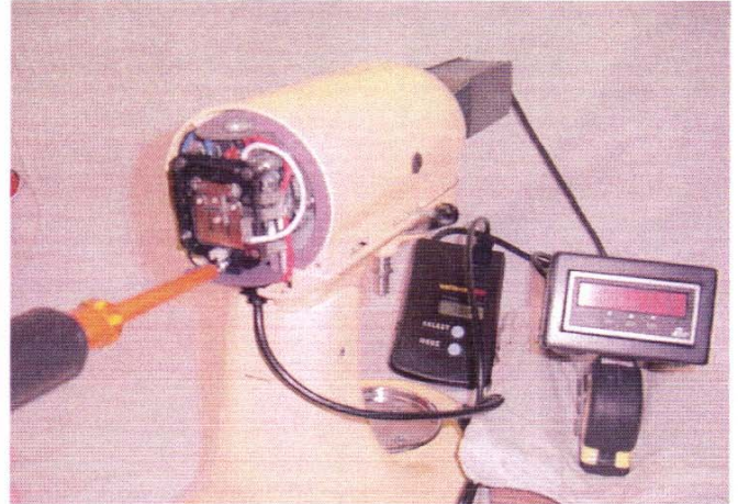
Fig. 79 Adjusting screw at the bottom of the control plate for speed # 6.
