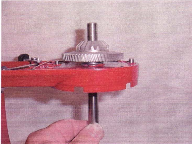
Fig. 54 Removal of vertical shaft from bottom cover.
