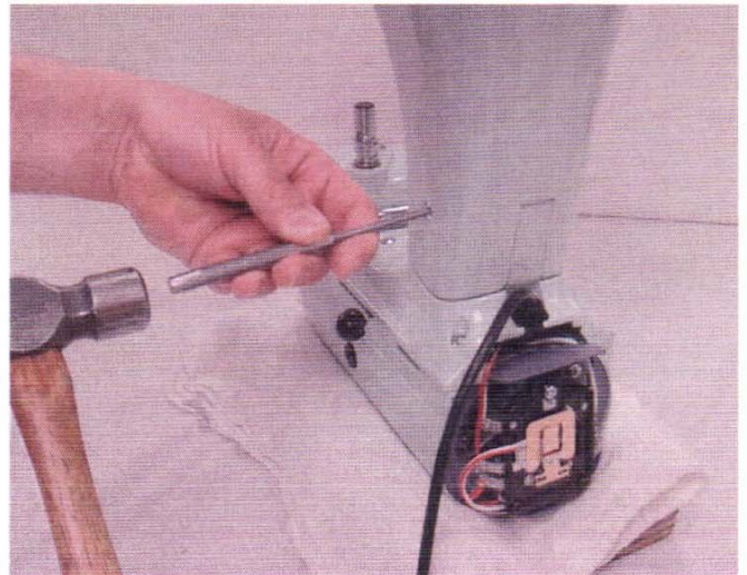
Fig. 4 A drift punch and hammer is used to drive out the hinge pin.
