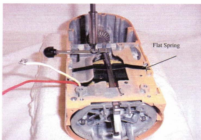
Fig. 24 The pivot screw and tension washer are removed with a phillips screwdriver.
