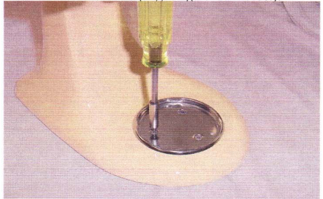
Fig. 72 The new cap is secured to the pedestal with three screws.
