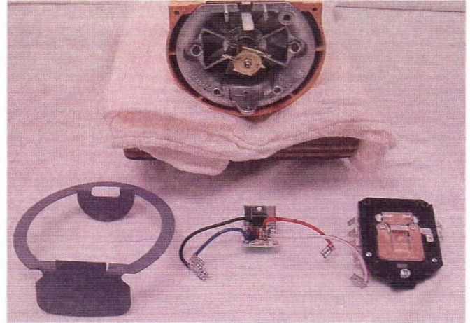
Fig. 20 Phase control or (triac) shown removed in lower center.
