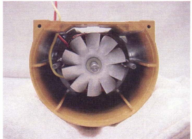
Fig. 39 Locating the armature into the gearcase-motor housing.
