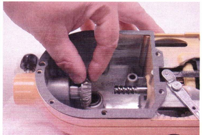
Fig. 13 The attachment hub bevel gear being removed from the mixer attachment hub bearing.
