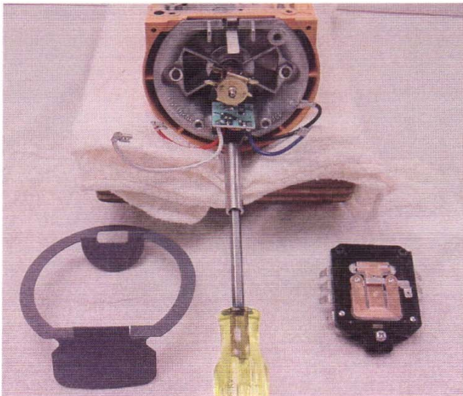
Fig. 19 Removal of the phase control (Triac) from the bearing bracket.
