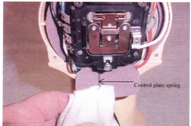
Fig. 76 Hold the control plate spring with a cloth to retain access for reassembly.
