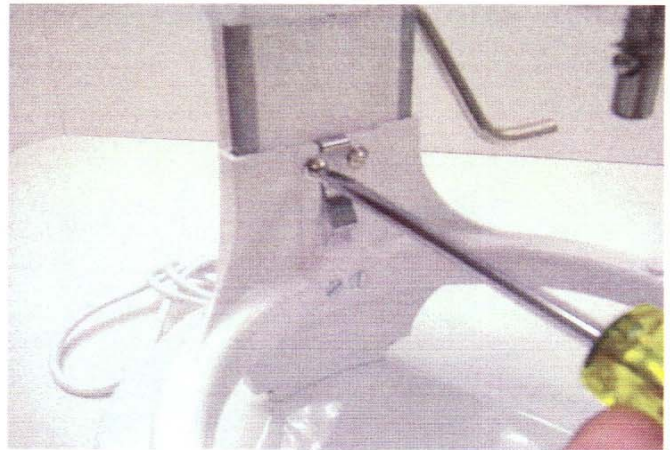
Fig. 95 Two #10-24 x 1/4" screws hold the bowl spring latch in place.
