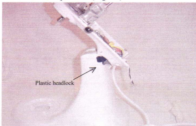
Fig. 74 A plastic headlock has been riveted to the pedestal of international export models. An international model is shown locked in the “inclined” position. This is obtained by the action of the spring loaded lock lever used on these models.
