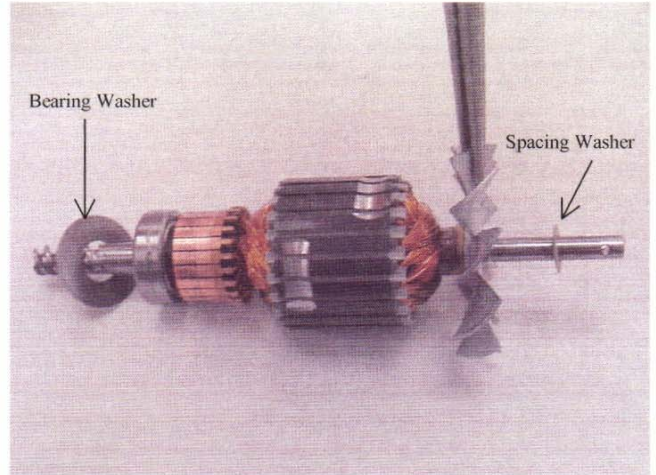
Fig. 38 Check the blades of the armature ventilating fan and straighten if bent.
