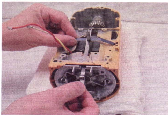
Fig. 25 Removing the speed control spring, flat spring and the speed control link assembly.
