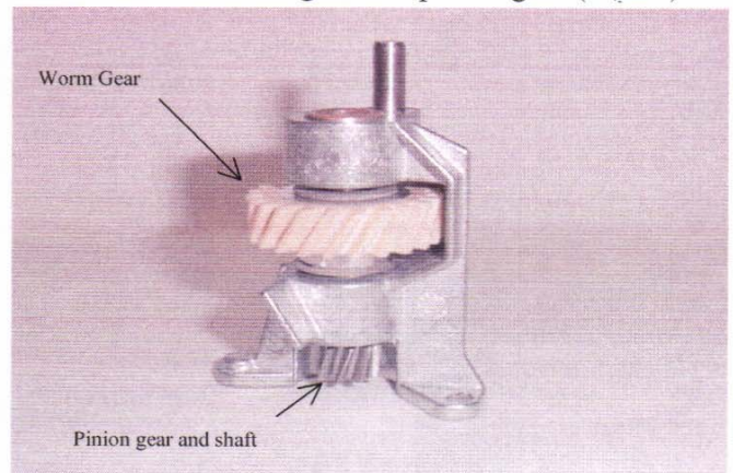
Fig. 56 Check worm gear and pinion before reassemble.
