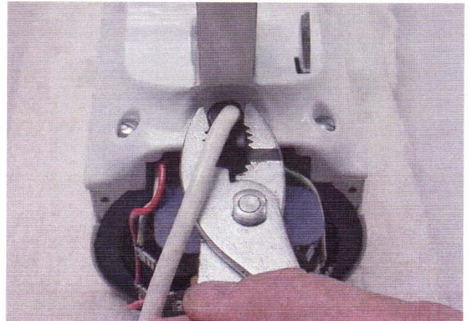
Fig. 9 Removal of Heyco strain relief using pliers.
