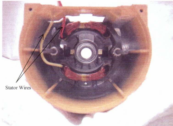
Fig. 31 Wire orientation inside the gearcase-motor housing
