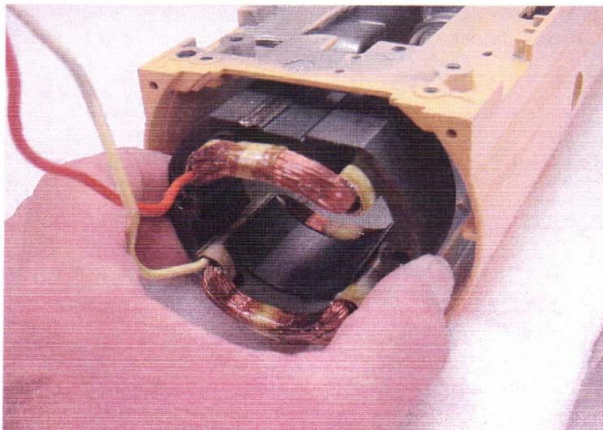
Fig. 32 The stator is shown being removed from the motor housing.
