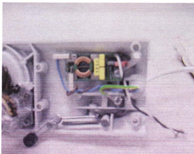
Fig. 75 International model bottom cover with R F filter and spring loaded lock lever.
