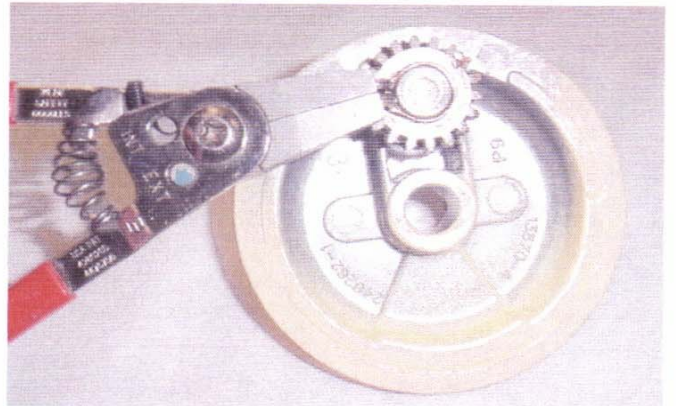
Fig. 64 Hold the agitator shaft and remove the retaining clip.
