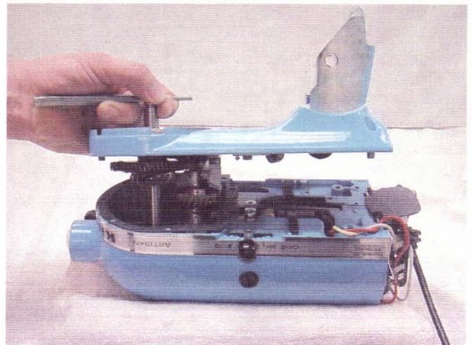
Fig. 60 Initial mating of bottom cover to gearcase - motor housing.
