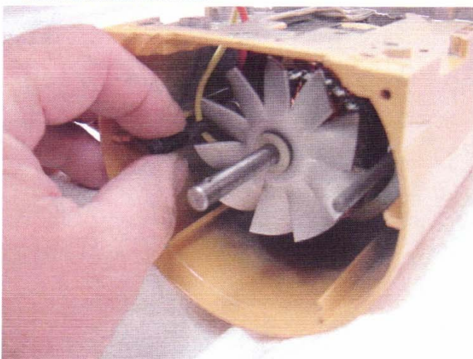
Fig. 28 The motor stud sleeve is shown being removed after bearing bracket removal.
