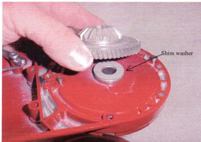
Fig. 55 Bevel center gear being lifted for inspection.
