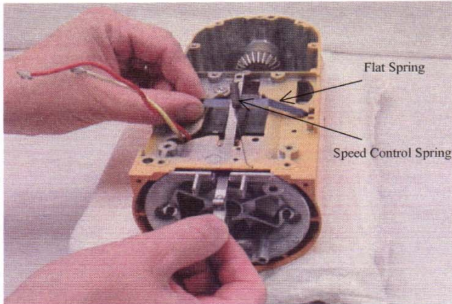
Fig. 43 Slide the speed control link over the flat spring and attach the speed control spring to the link.
