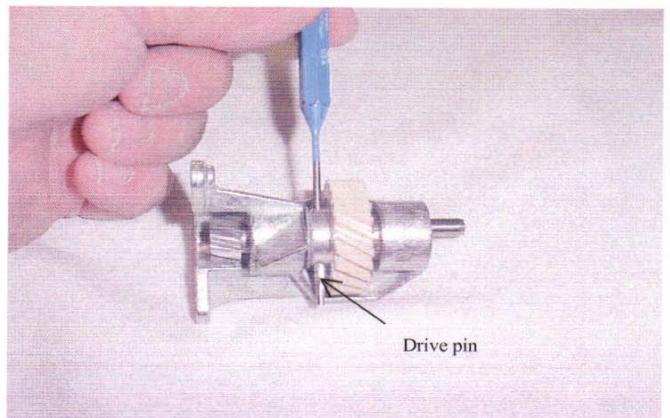
Fig. 57 The drive pin must be removed to change the gears.
