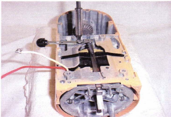
Fig. 44 Securing the pivot screw to the gearcase after placing the tension washer.
