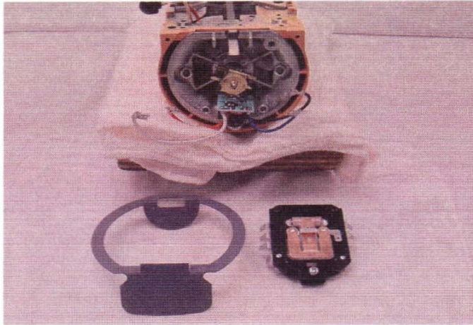
Fig. 18 Mixer housing with end seal and control board removed.
