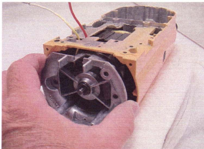
Fig. 27 Bearing bracket being removed after two #10-24 nuts have been removed.
