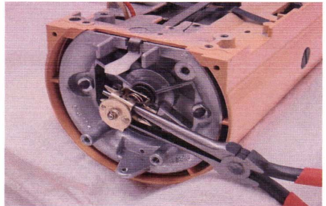
Fig. 21 Needle nose plier used to pry governor off the motor shaft.
