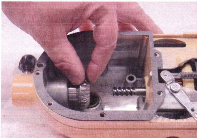
Fig. 51 The attachment hub bevel gear being pushed into the attachment hub bearing from inside the gearcase.
