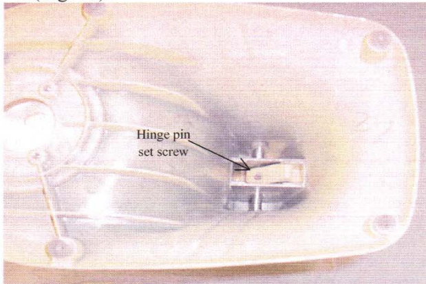
Fig. 70 The set screw in the bottom of the pedestal should clear the hinge pin.
