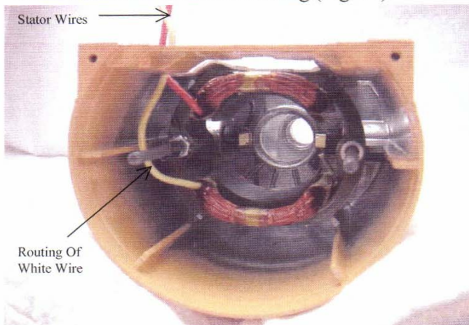
Fig. 37 Route the two stator wires through the slot in the motor housing.
