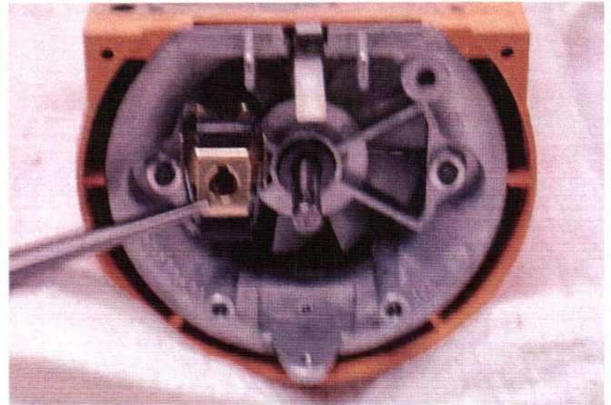
Fig. 45 The governor shown before being placed on the motor shaft.
