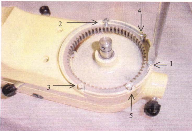
Fig. 62 Tighten the five special screws evenly to 18-20 in. lbs. torque using the sequence shown.
