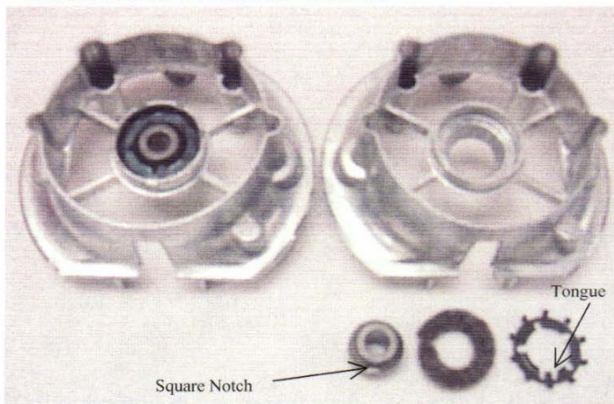
Fig. 40 Bearing bracket assembled & unassembled
