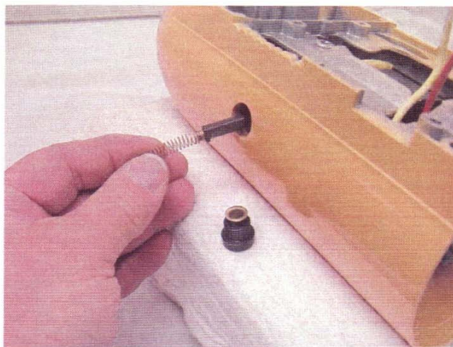
Fig. 29 the brush holder caps are loosened to access brushes for removal. Make sure to mark orientation.
