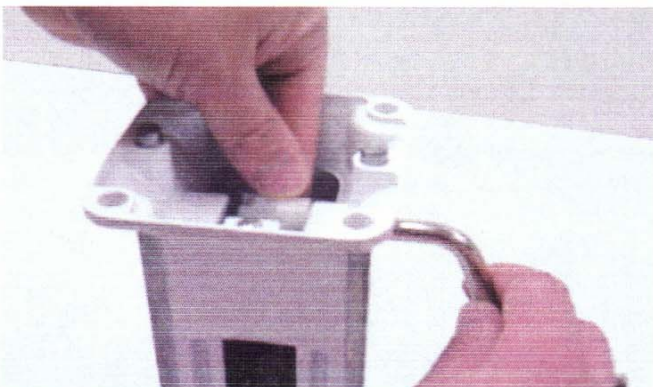
Fig. 90 With the roll pin removed, pull out the handle.
