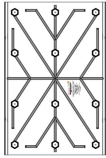
UNDERSIDE VIEW
