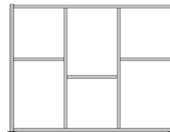
Model Number SW7558-3 FULL UNIT (2 SUPPORT POSTS)
