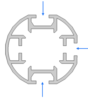
triple slotted corner post for a 3-way connection
