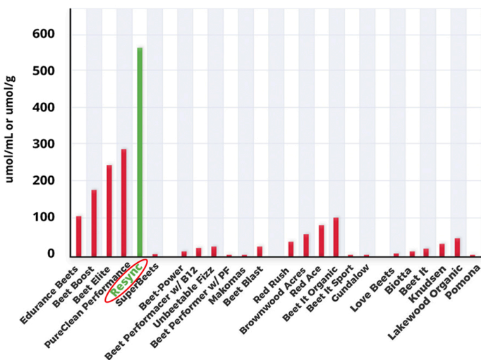
\text{No}_3 content of beet juice products
