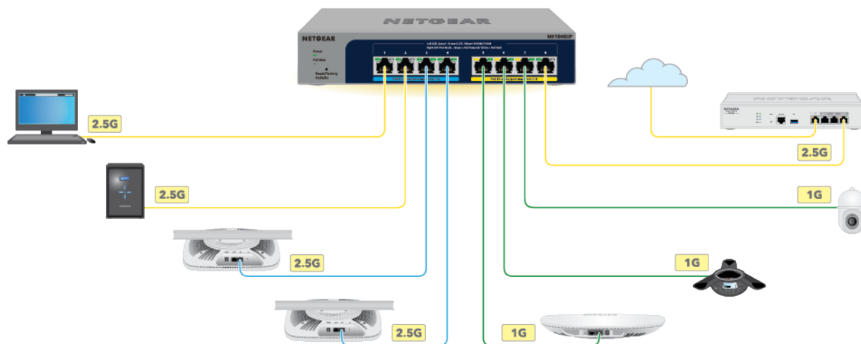
Figure 1. Example connections
