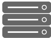
LEAPS Server
