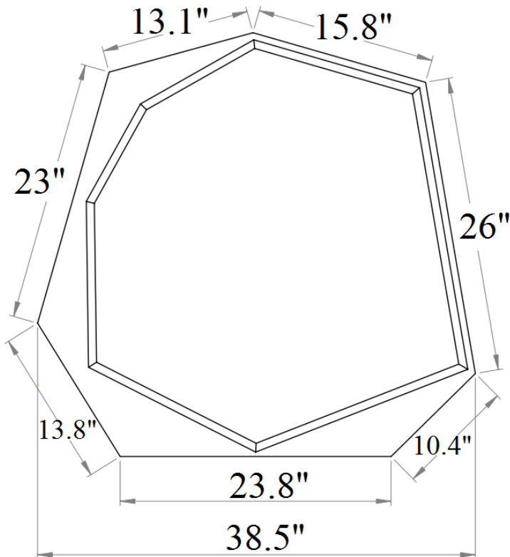
Front View
