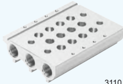
MANIFOLD RAIL VABM FOR INDIVIDUAL VALVE VUVG-L WITH SEAL VABM-L1-10X 10 MM SIZE
