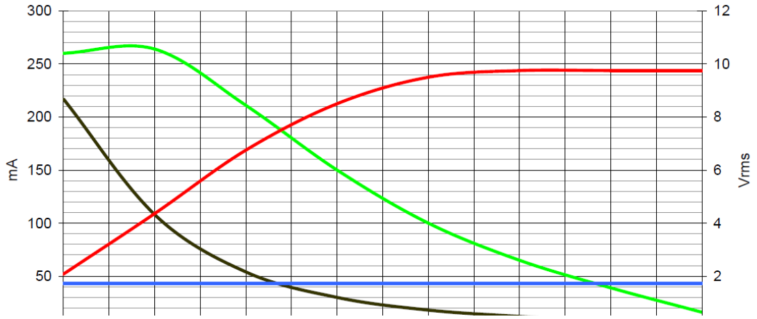
Extreme Power: Current / Voltage vs Impedance
