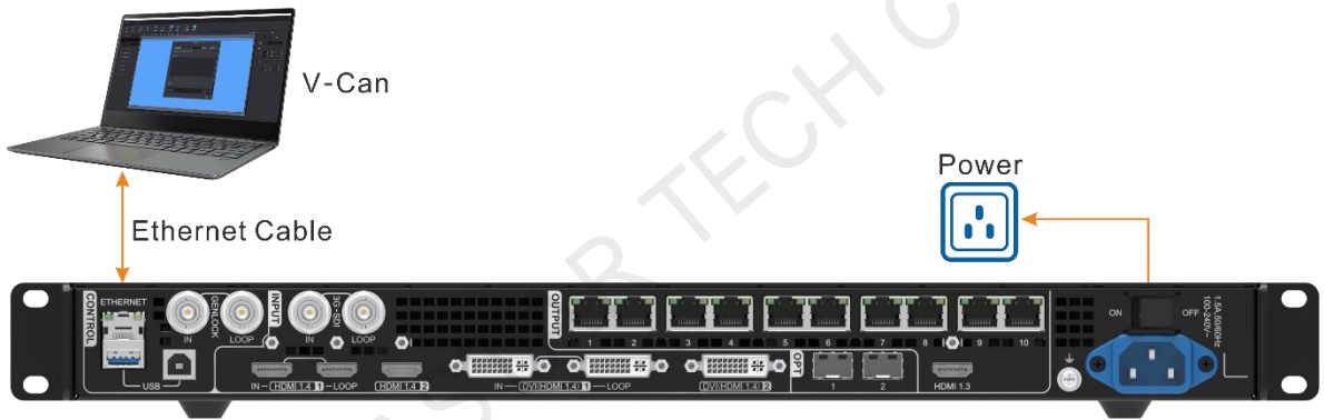
Figure 6-1 Hardware connection
