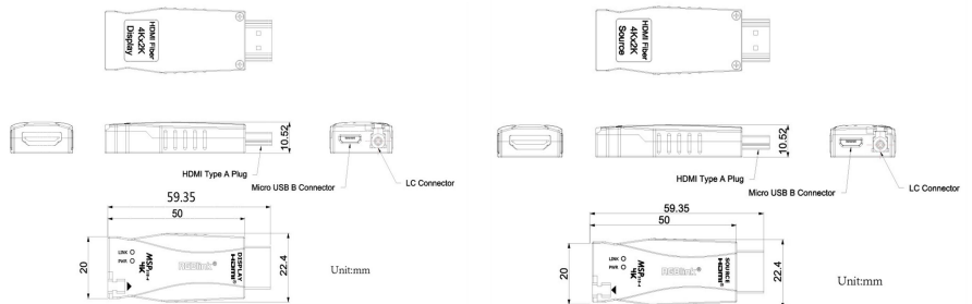
MSP 318-4 Transmitter
