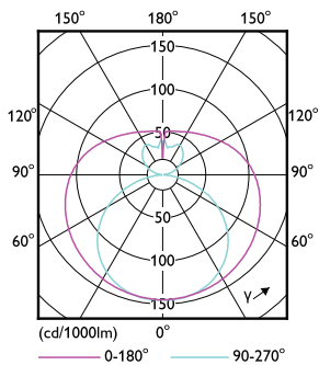
Light Distribution Diagram - CorePro LEDtube 1200mm 17.6W 840 T8 AU
