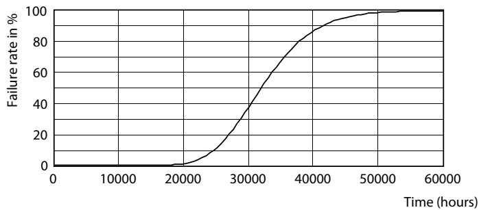
Life Expectancy Diagram - CorePro LEDtube 1200mm 17.6W 840 T8 AU
