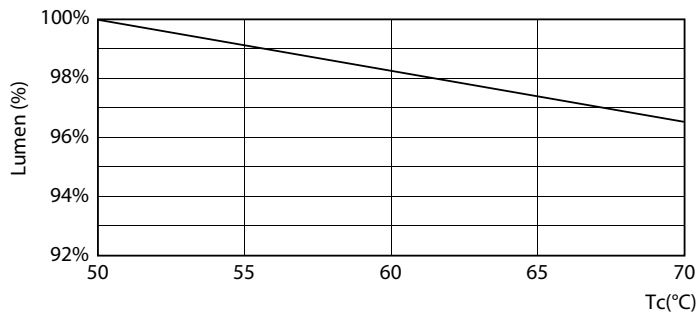
Lumen Maintenance Diagram - CorePro LEDtube 1200mm 17.6W 840 T8 AU
