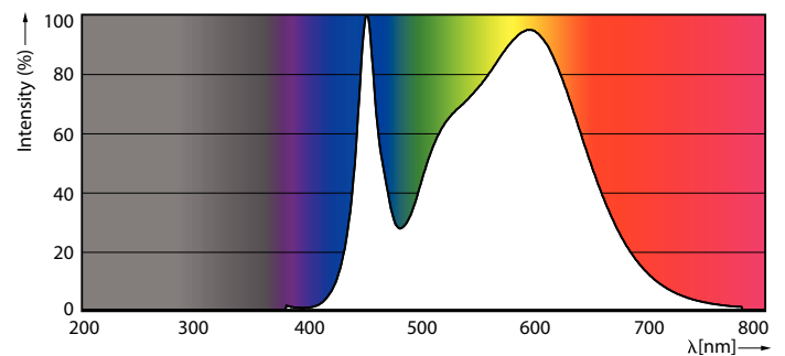
Spectral Power Distribution Colour - CorePro LEDtube 1200mm 17.6W 840 T8 AU
