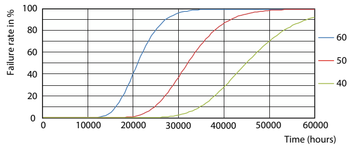
Life Expectancy Diagram - CorePro LEDtube 1200mm 17.6W 840 T8 AU
