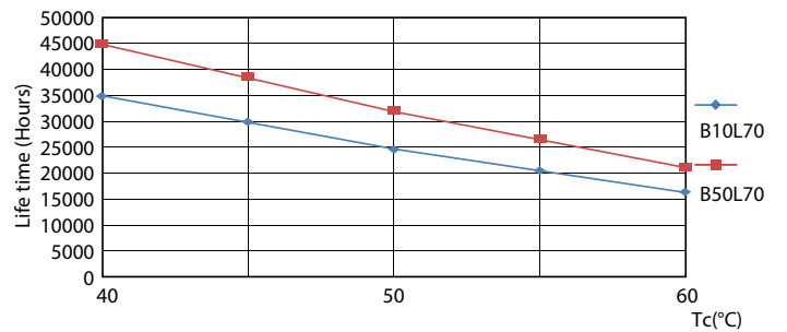
Life Expectancy Diagram - CorePro LEDtube 1200mm 17.6W 840 T8 AU
