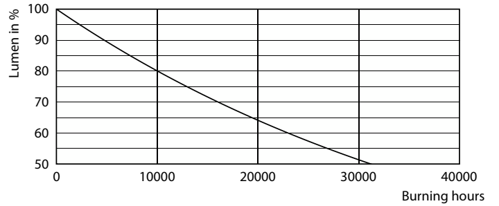
Lumen Maintenance Diagram - LEDBulb 8.5-60W E27 2700K D 1PF/6 AU
