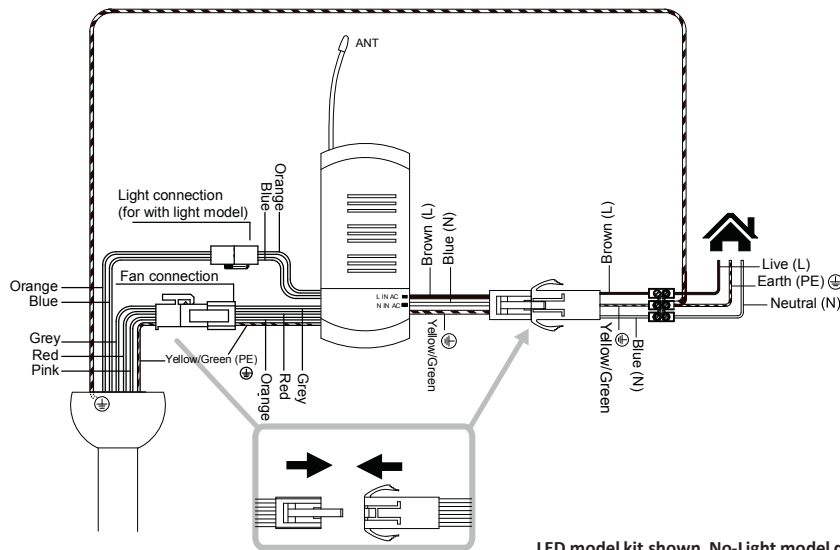
LED model kit shown, No-Light model does not contain 'Light Connection' wires.
