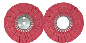
9" RED DOUBLE STITCHED WITH CENTER PLATE PART# FAW9X3X5/BN2-16PPT2-2RS 9" RED DOUBLE STITCHED CENTERLESS PART# FAW9X3N2-16PPT2-2RS
