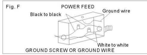
Wiring Connection in J-box for low voltage
