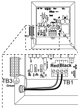
Figure C Connections (North American 60 Hz 240 VAC Connection Models)
