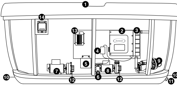
Figure 6.0c Equipment Area
