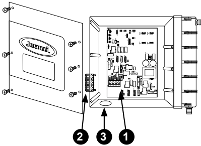
Figure 6.0d Terminal Block Connection
