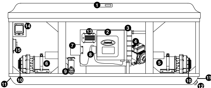
Figure 6.0a Equipment Area
