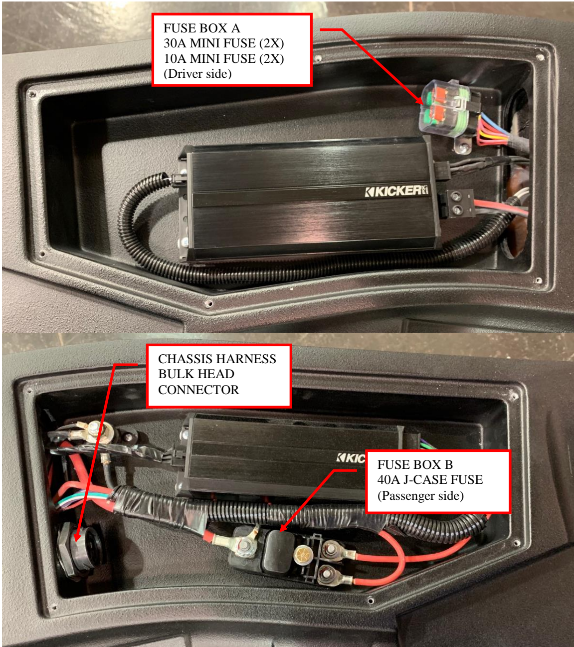
Figure 2: Fuse location.
