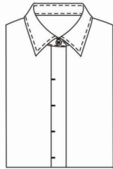
91H4 Exposed hidden placket with bartack
