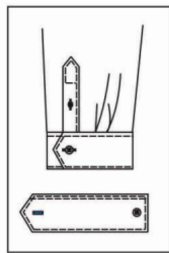
9774 Pointed cuff one button one buttonhole
