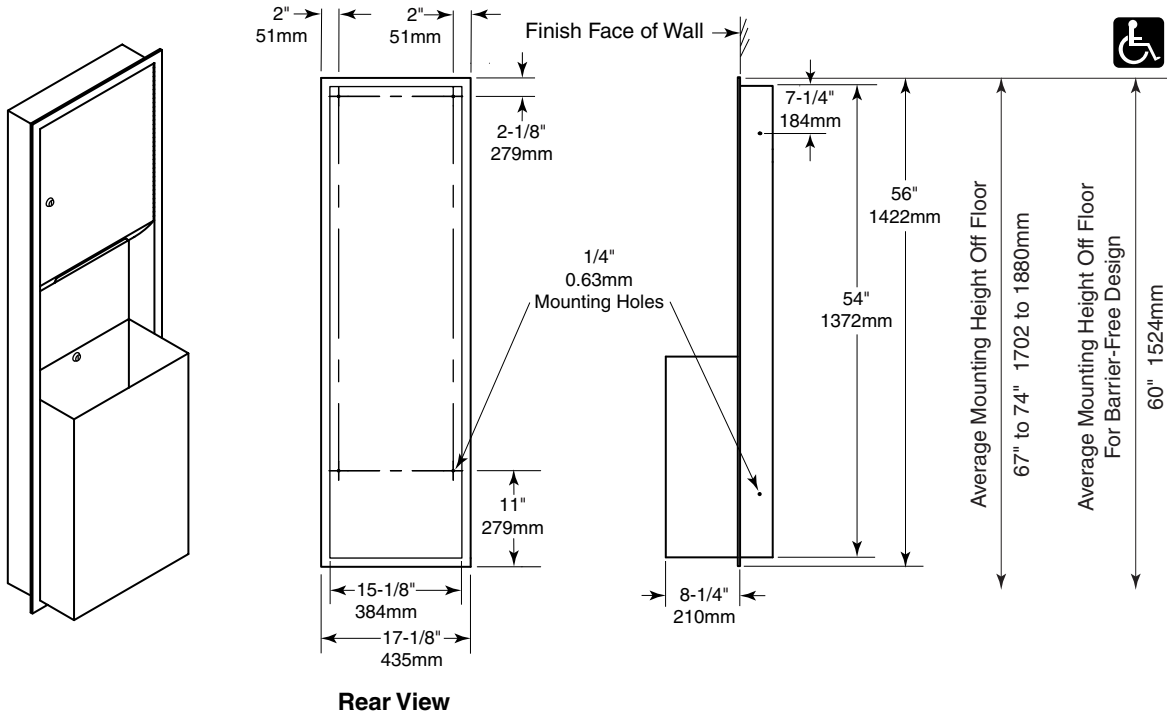
Rear View
