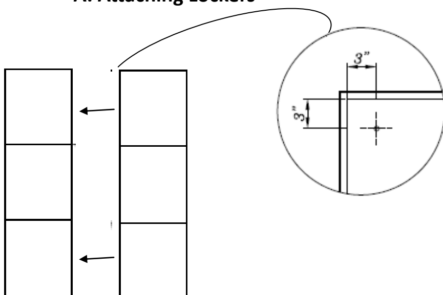
A. Attaching Lockers
