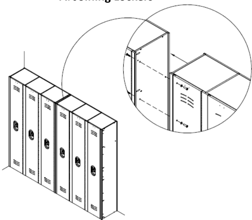
A. Joining Lockers
