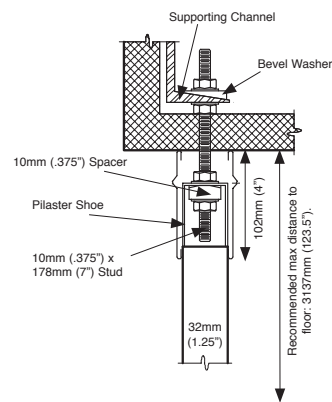
section detail B-B
