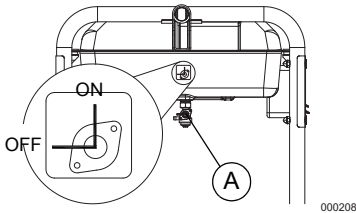
Figure 3-2. Fuel Shut-off Valve
