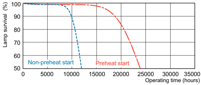
Life Expectancy Diagram - F35T5/841 40PK
