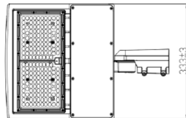
WL-PLF-100W/150W
