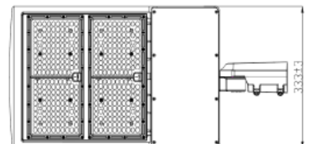
WL-PLF-300W
