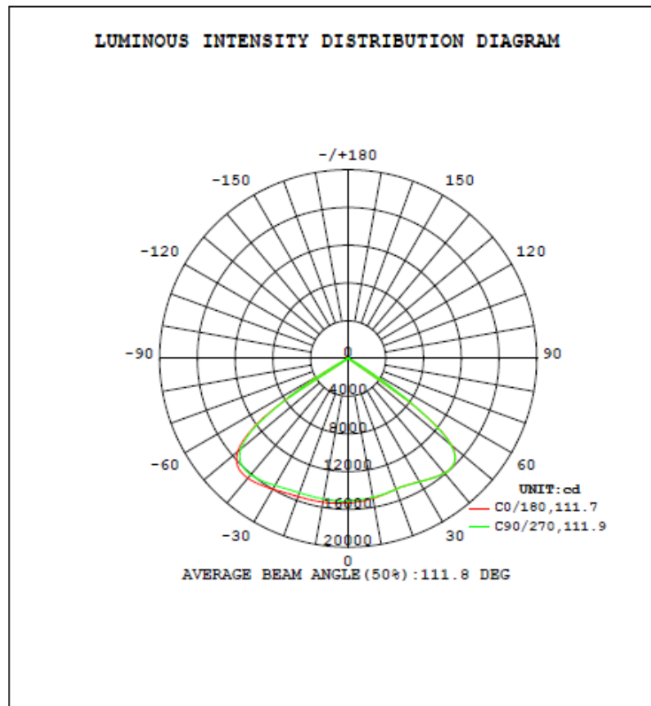
Saturn 240W 5K 110° Optic
