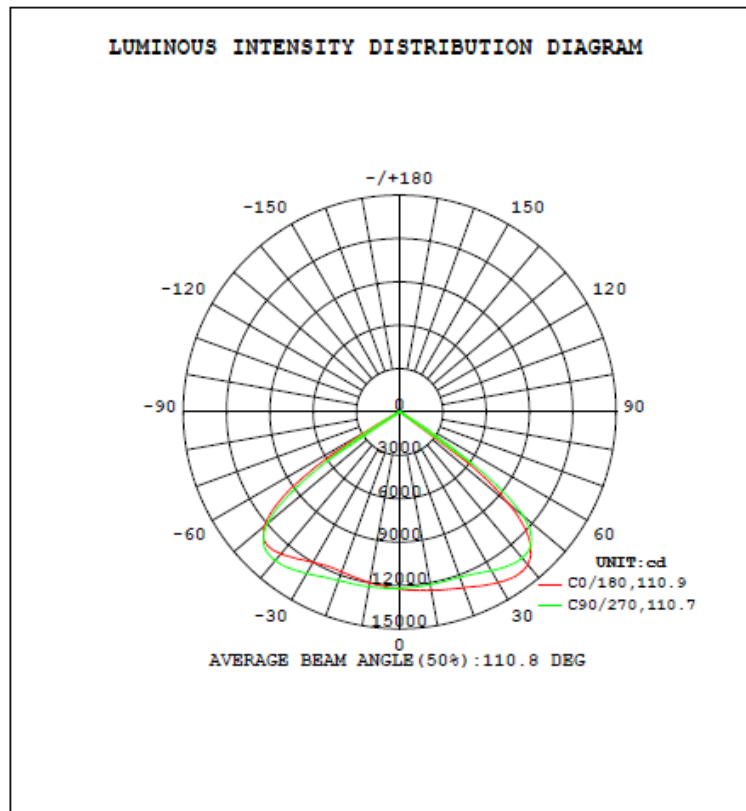
Saturn 200W 5K 110° Optic
