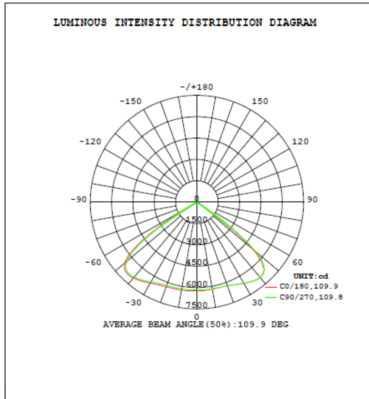
Saturn 100W 5K 110° Optic
