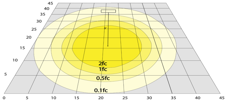
Area 45'x 45' Mounting Height: 9'
