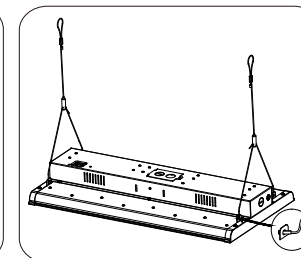
2. Insert the hook into the slotted holes as shown above.
