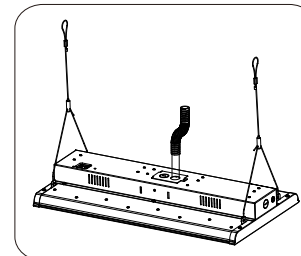
4. Make wiring connections with terminal cap (see wiring diagram below).
