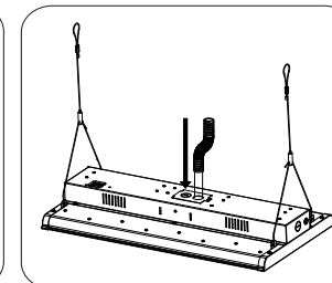
5. Insert the terminal cap and wire into the driver box.
