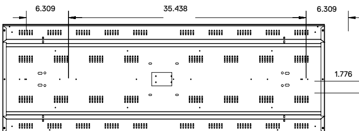
TONG HANGERS HOLE DISTANCES
