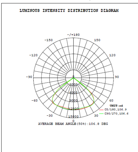
200W 4K 110° Optic
