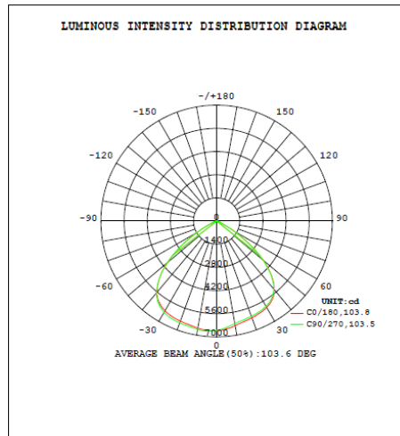
100W 4K 110° Optic
