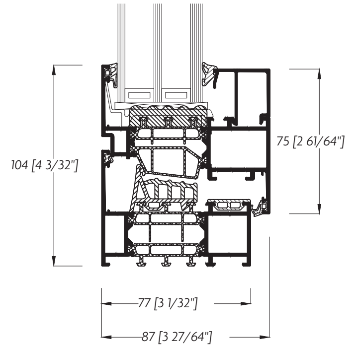
MasterLine8
