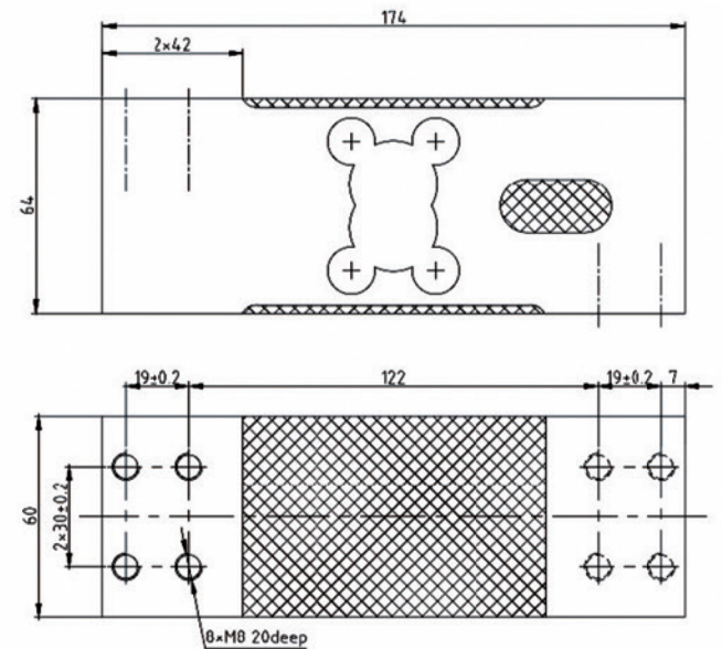
Outline dimensions (in millimeters)
