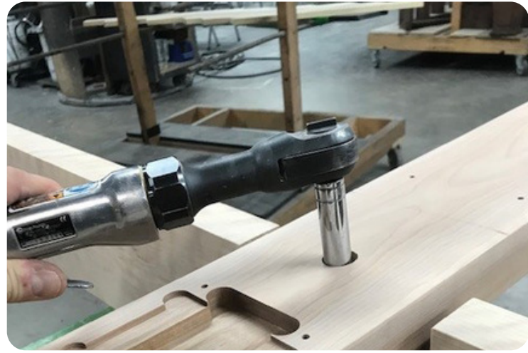
7 Fix the net crossmember with 3/8"-16 x 1 3/4" hexagonal bolts and 13/32" plat wachers.
