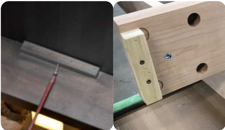
18 Attach the frame to the playing surface and cross members with wood screws #8 x 1 1/4" round headed. Also use the large holes underneath the net crossmember to fix the surface.
