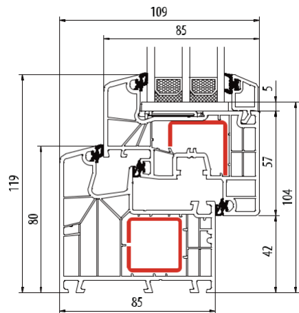
Ideal 8000 Classic-line
