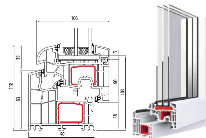
BluEvolution 92 Round-line
