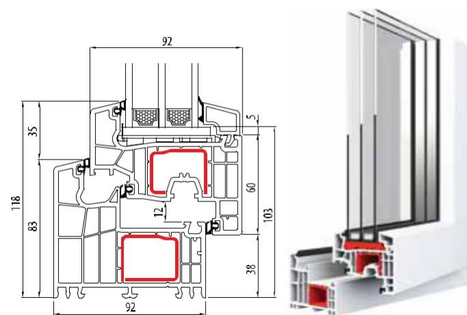
BluEvolution 92 Classic-line
