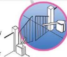
Dual Leaf Gate Built in Open/Close Delay 2-Wire Master/Slave Accessories Connect to Master or Slave Operator
