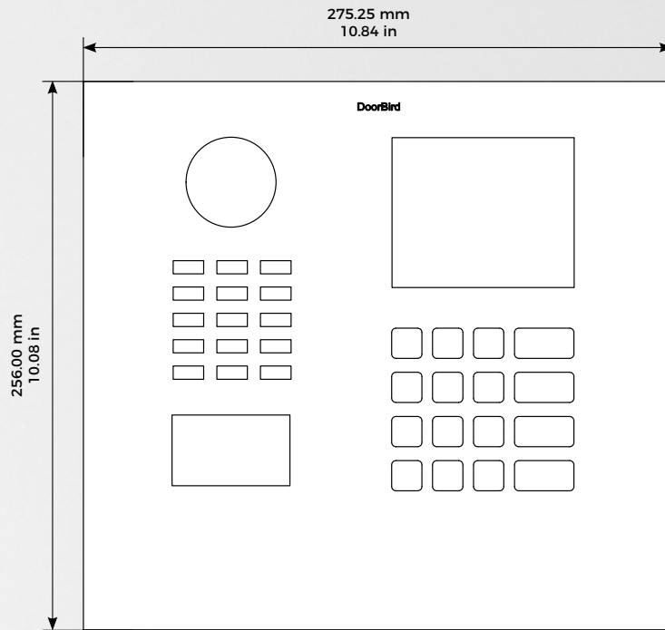
Front panel
