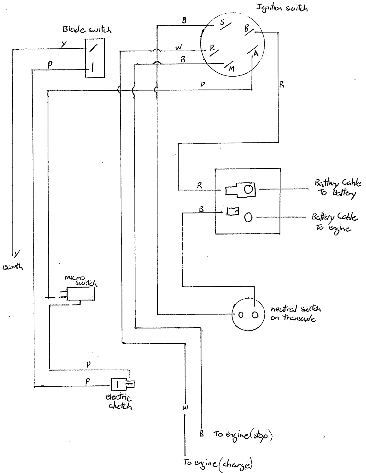
Wiring Diagram. Tiger.
