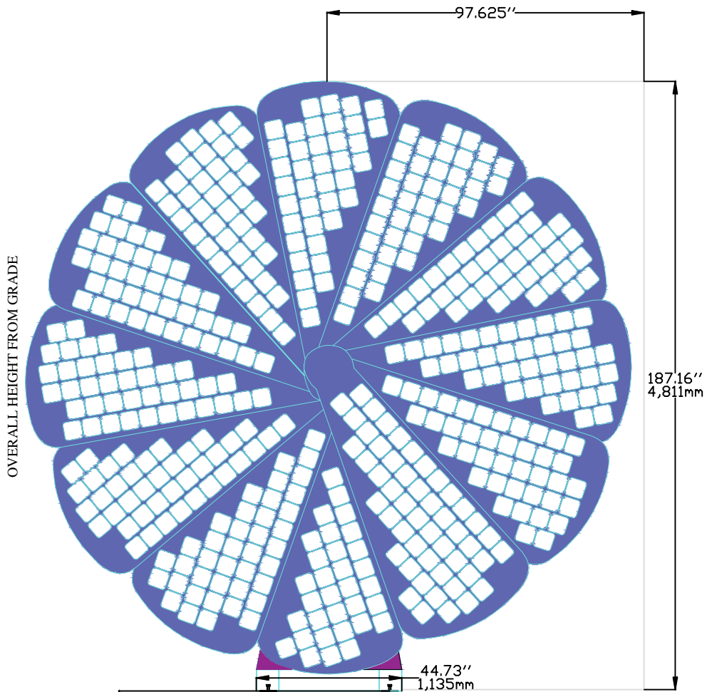
FRONT ELEVATION
