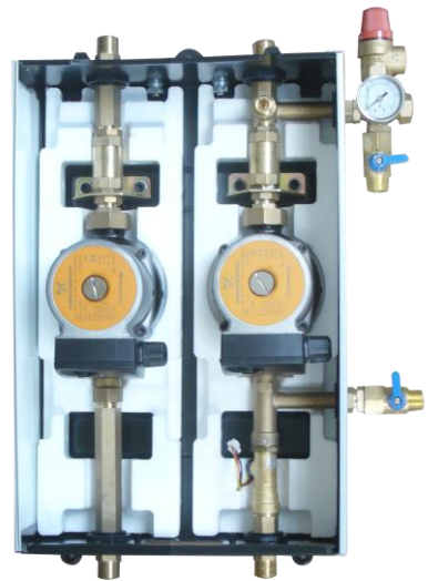
SR962P built-in DHW pump picture
