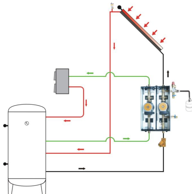
Double pump station for auxiliary heating application
