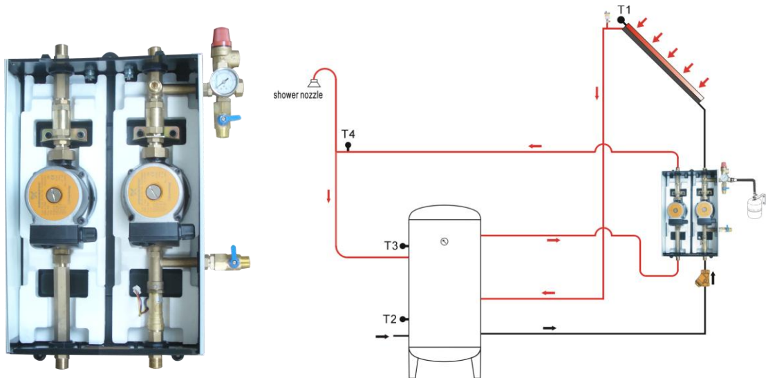
Double pump station for DHW application
